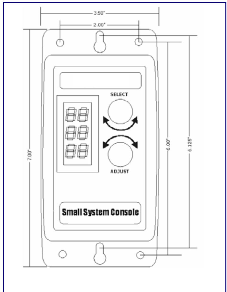
Mechanical Dimensions – Front View
