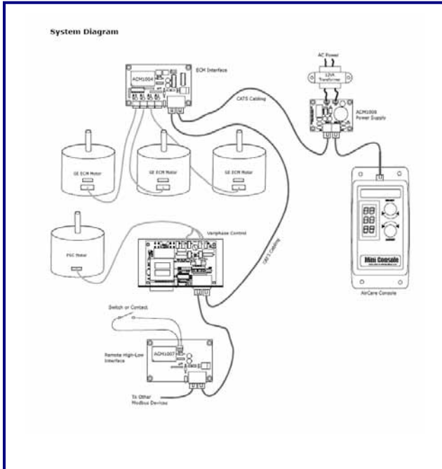
ACC1-xxx System Diagram (EC & AC types)
