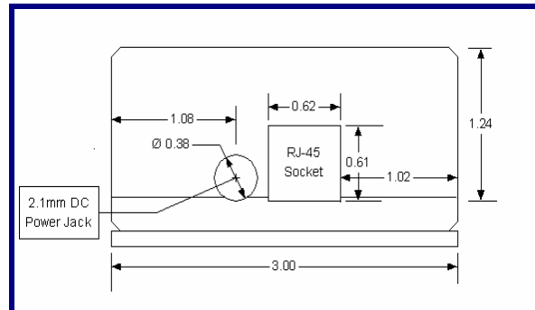
Mechanical Dimensions -Top View
