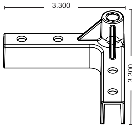
2 Way Corner
