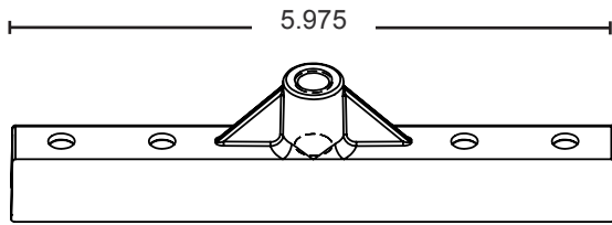
2 Way Connection
