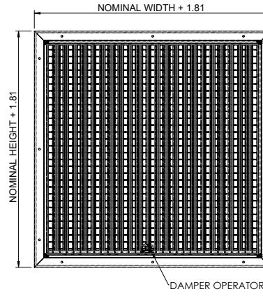
FACE VIEW
