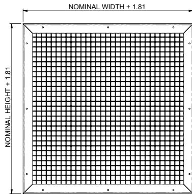
FACE VIEW
