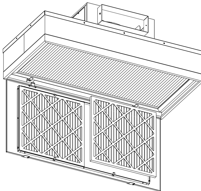
Figure 4: Prefilter Replacement
