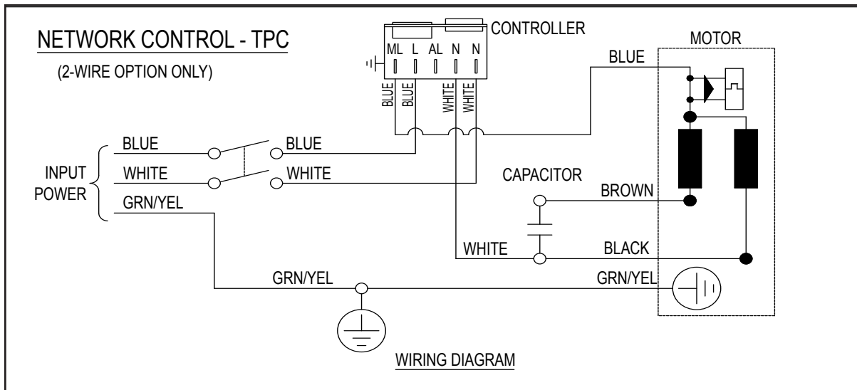
Figure 13: Wiring Diagram (TPC)
