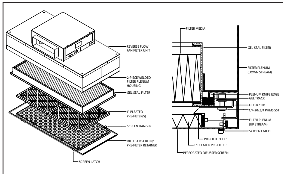
Figure 10: RSR Filter Replacement
