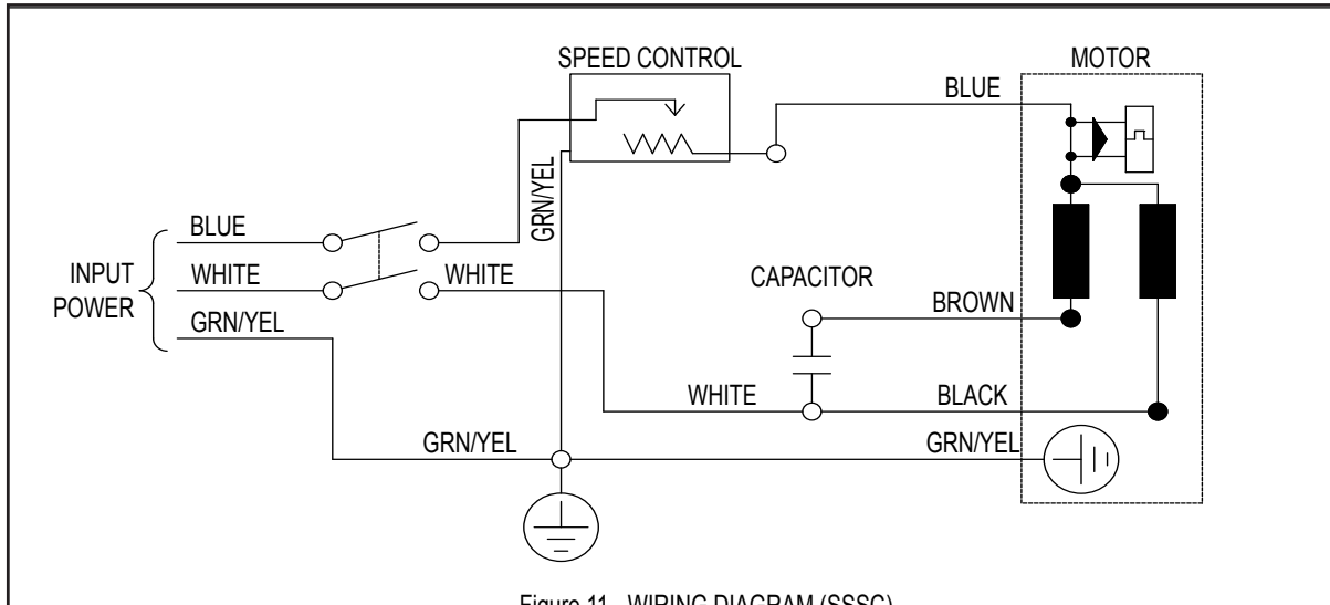
Figure 11: WIRING DIAGRAM (SSSC)
